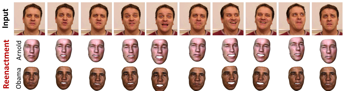
Fig. 8. Facial Reenactment: We retarget the rigid and non-rigid head motion of an input actor (top row) to the high-quality 3D rigs of ARNOLD OLD (middle) and OBAMA (bottom). Note that the target actor’s characteristics are maintained, since we regress the detail layers.
