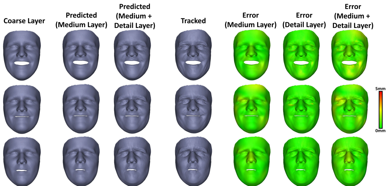
Fig. 12. Evaluation of the prediction accuracy: Our novel sparse regression strategy infers high-quality medium and fine-scale detail layers given a novel expression. Note that we compare quantitatively to the tracked ground truth reconstruction which is accurately reproduced. The prediction error of the medium and detail layer together is always smaller than 3.5mm (1mm mean and 0.16mm standard deviation). The error is mainly explained by residuals in the medium layer, while the error of the detail layer is mostly negligible ( < 0.4\text{mm} on average).
