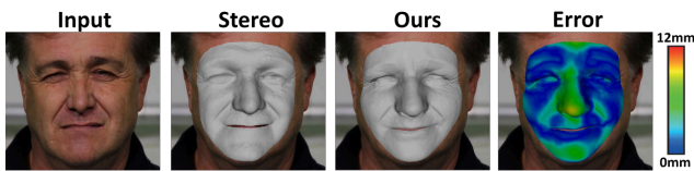
Fig. 10. Geometric Accuracy: Our monocular approach obtains similar quality (1.8mm mean error) to that of the high-quality binocular approach of Valgaerts et al. [2012].
