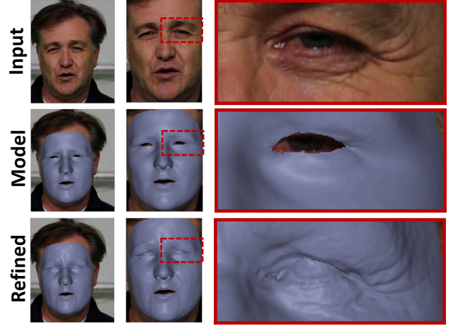
Fig. 4. Shape Refinement: We exploit shading cues in the input image (top) to augment the medium-scale model (middle) with fine-scale static and transient surface detail (bottom).
