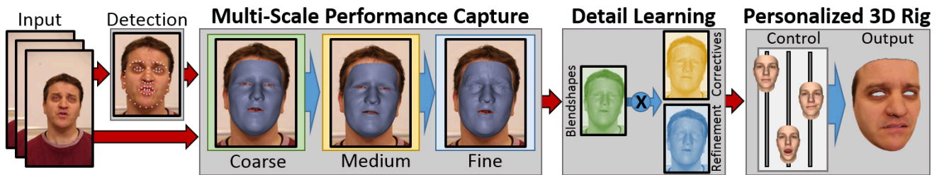
Fig. 2. Pipeline Overview: Starting from monocular video data, we first reconstruct the actor’s identity and motion parameters based on a novel tracking energy, resulting in a multi-layer 3D rig. Finally, we learn the coupling between coarse-scale expression changes and medium as well as fine-scale surface detail.
