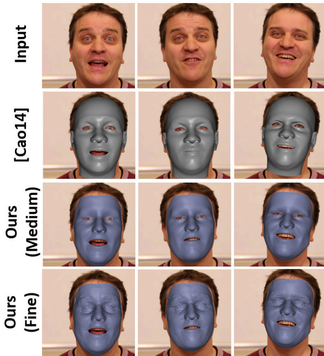
Fig. 11. State-of-the-art comparison to [Cao et al. 2014]: Monocular input (first row), result obtained by the approach of Cao et al. [2014] (second row), our medium-scale result (third row) and our final fine-scale reconstruction (forth row). Note that our medium-scale result matches the actor more closely and the fine-scale reconstruction adds even more realism.
