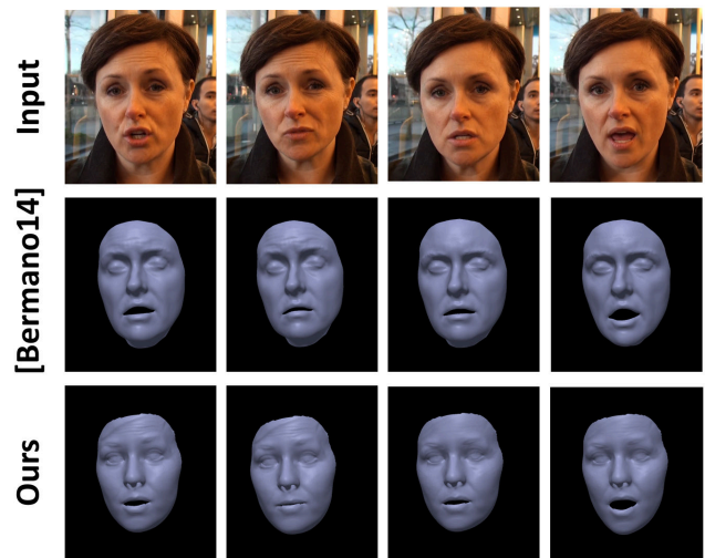
Fig. 16. State-of-the-art comparison to the approach by [Bermano et al. 2014]: Our approach obtains predicted correctives and fine-scale detail comparable to Bermano et al. ’s method, which requires a tailor-made set of training sequences to enhance fine-scale detail and expressiveness.
